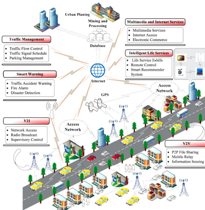
Figure 8. Architecture and applications of VSN in a smart city (Wang, et al., 2017).
